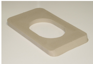
Tank-to-Bowl Gasket for Flapperless Models Niagara Part #: C2216-28
